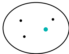
Element
