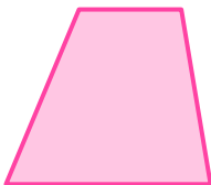
Trapez
