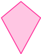
Deltoid
