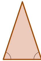
Triangelu isoszele
