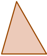
Triangelu zorrotz
