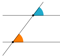
Corresponding angles
