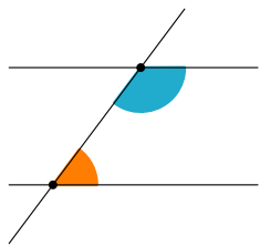
Interior angles
