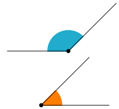
Supplementary angles
