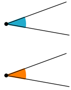
Equal angles
