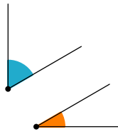
Complementary angles
