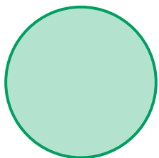
Disc
