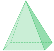
Piramide
