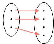
Injective (one-to-one)
