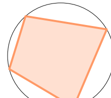
Cyclic polygon
