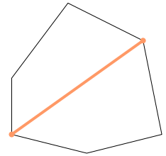
Diagonal
