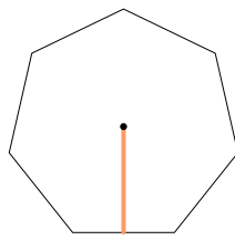
Apothem
