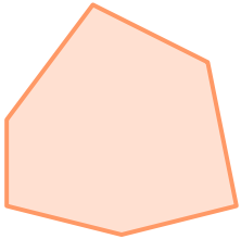
Convex polygon
