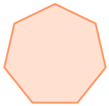
Regular polygon
