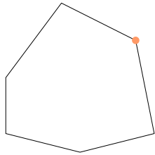
Vertex (Corner)
