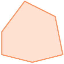
Polygone convexe
