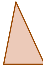
Triangle scalène
