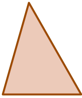
Triangle acutangle
