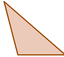
Triangle obtusangle
