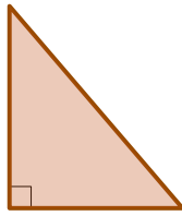
Triangle rectangle
