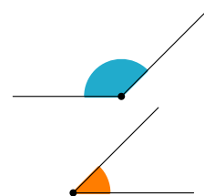
Angoli supplementari
