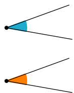
Angoli congruenti
