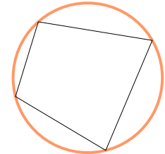
wài jiē yuán
