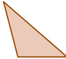
dùn jiǎo sān jiǎo xíng
