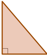
zhí jiǎo sān jiǎo xíng
