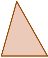
ruì jiǎo sān jiǎo xíng
