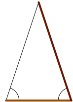
dǐ biān, yāo
