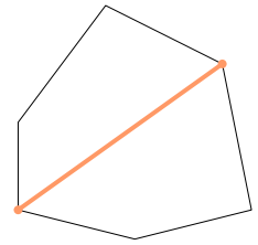
Diagonal
