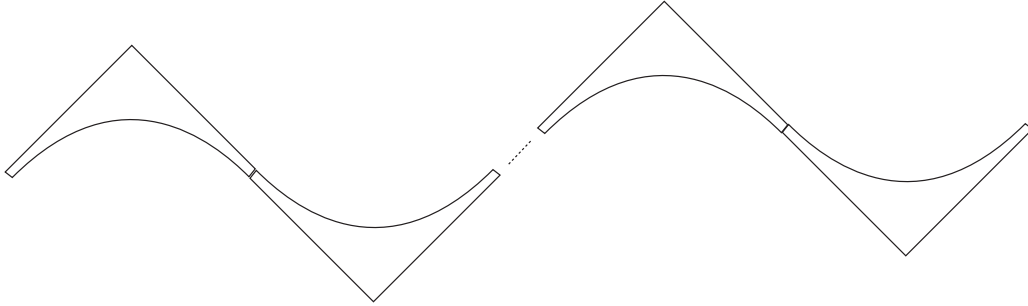
FIGURE 5. n - 4 l -pentagons pasted along short edges
