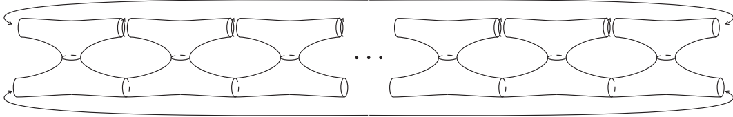
FIGURE 17. Genus g
