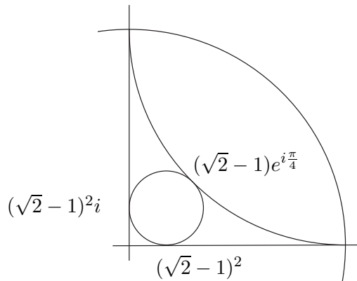
FIGURE 2. The hyperbolic triangle of vertices 0, 1 and i
