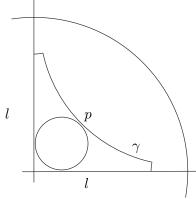
FIGURE 4. The l -pentagon
