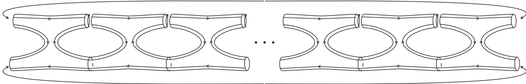
FIGURE 18. The winning geodesic for genus g
