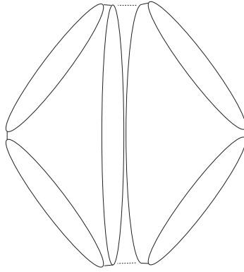
FIGURE 14. A surface obtained by pasting l -pants
