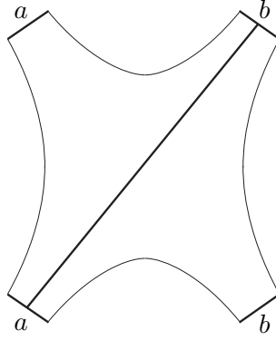
FIGURE 9. When a and b are both short
