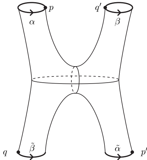
FIGURE 15. Genus 2
