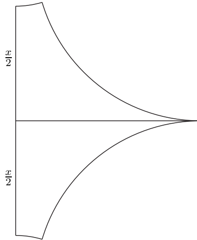
FIGURE 12. An symmetric ideal pentagon
