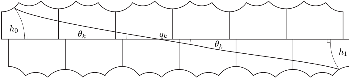
FIGURE 20. \mathcal{X}_{\gamma_i} seen 3 times
