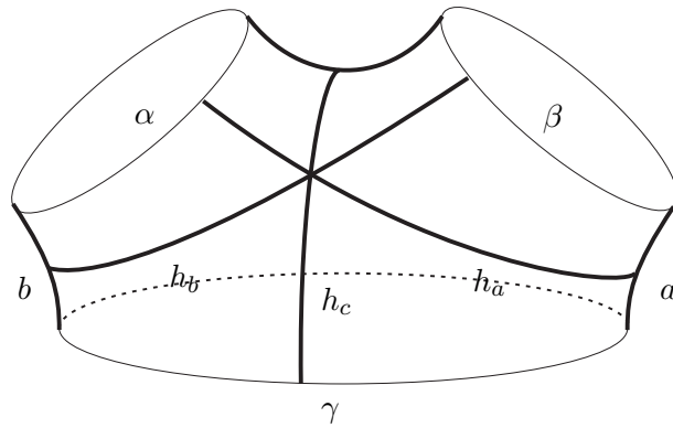
FIGURE 7. \mathcal{Y} and certain paths
