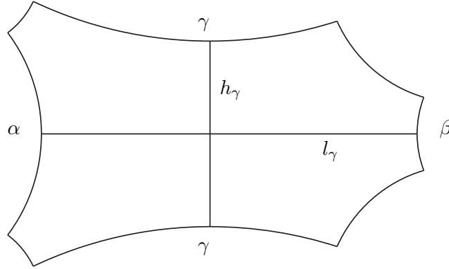
FIGURE 13. A Y -piece cut along two common perpendiculars
