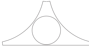
FIGURE 10. A hexagon used to obtain a Y -piece containing the smallest possible disk
