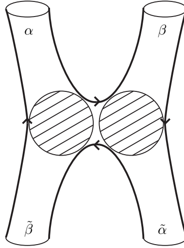
FIGURE 16. The winning geodesic for genus 2
