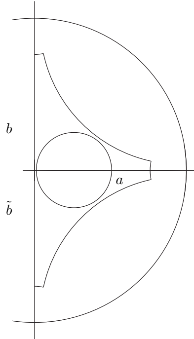
FIGURE 6. The disk of radius \rho_s
