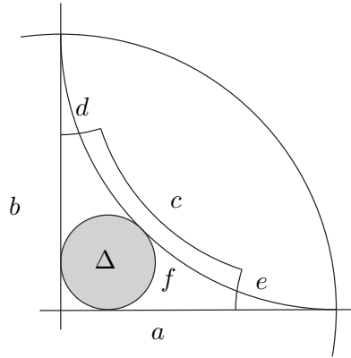
FIGURE 3. A hyperbolic pentagon
