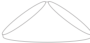
FIGURE 11. An l -pants
